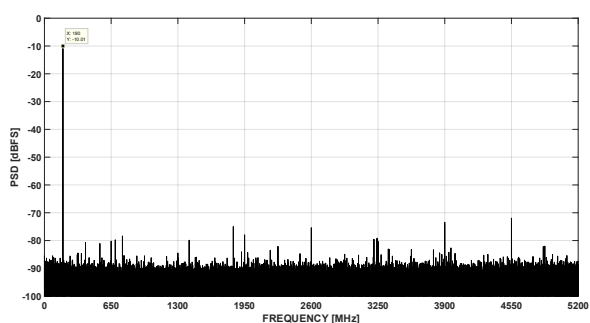
图 7-27. FFT at F_{in} = 180\text{MHz} , 10.4GSPS (0.8Vpp FS, -10 dBFS)
