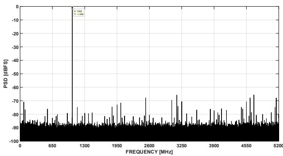
图 7-21. FFT at Fin = 1.05GHz, 10.4GSPS (0.8Vpp FS, -1 dBFS)
