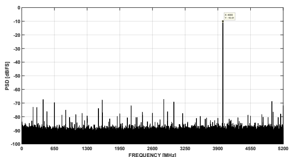
图 7-31. FFT at F_{in} = 4\text{GHz} , 10.4GSPS (0.8Vpp FS, -10 dBFS)
