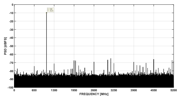
图 7-14. FFT at Fin = 1.05GHz, 10.4GSPS (0.5Vpp FS, -10 dBFS)
