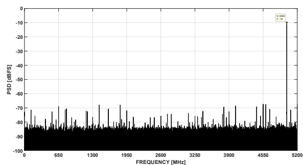
图 7-18. FFT at Fin = 5GHz, 10.4GSPS (0.5Vpp FS, -10 dBFS)
