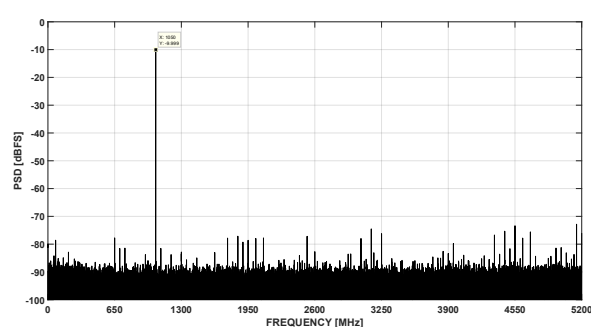
图 7-28. FFT at F_{in} = 1.05\text{GHz} , 10.4GSPS (0.8Vpp FS, -10 dBFS)
