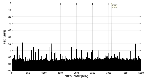
图 7-24. FFT at Fin = 4GHz, 10.4GSPS (0.8Vpp FS, -1 dBFS)
