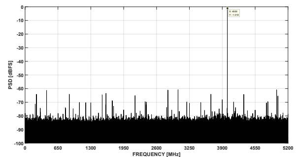
图 7-10. FFT at F_{in} = 4\text{GHz} , 10.4GSPS (0.5Vpp FS, -1 dBFS)
