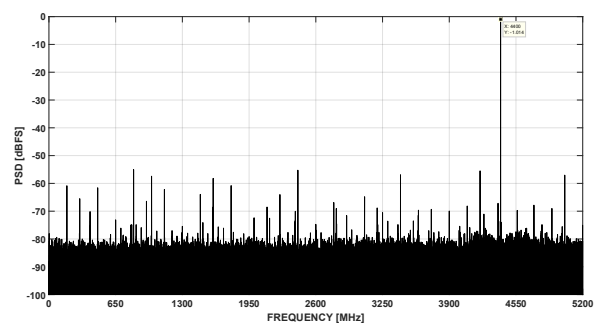
图 7-26. FFT at Fin = 6GHz, 10.4GSPS (0.8Vpp FS, -1 dBFS)
