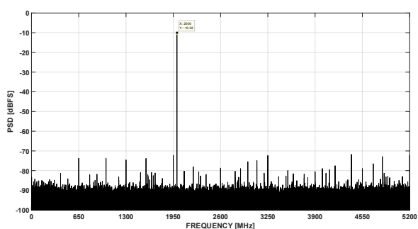
图 7-29. FFT at F_{in} = 2\text{GHz} , 10.4GSPS (0.8Vpp FS, -10 dBFS)
