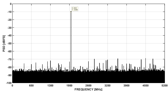
图 7-15. FFT at Fin = 2GHz, 10.4GSPS (0.5Vpp FS, -10 dBFS)
