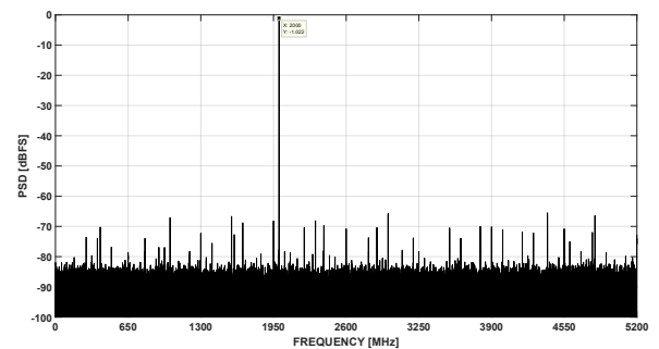
图 7-8. FFT at F_{in} = 2\text{GHz} , 10.4GSPS (0.5Vpp FS, -1 dBFS)
