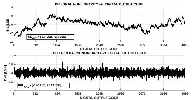
图 7-4. INL/DNL at F_{in} = 180\text{MHz} , 10.4GSPS (0.8Vpp FS)
