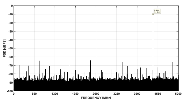
图 7-33. FFT at F_{in} = 6\text{GHz} , 10.4GSPS (0.8Vpp FS, -10 dBFS)
