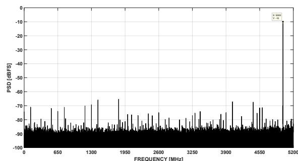
图 7-32. FFT at F_{in} = 5\text{GHz} , 10.4GSPS (0.8Vpp FS, -10 dBFS)
