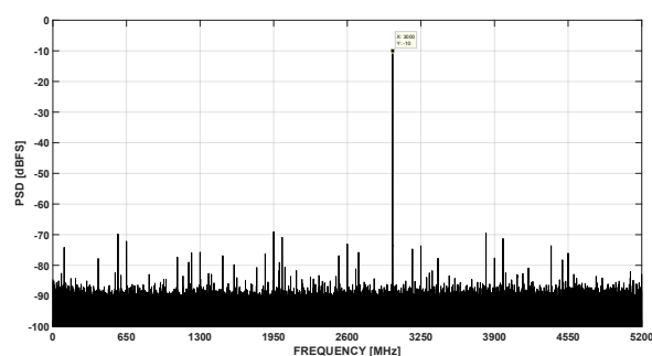
图 7-30. FFT at F_{in} = 3\text{GHz} , 10.4GSPS (0.8Vpp FS, -10 dBFS)
