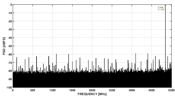
图 7-11. FFT at Fin = 5GHz, 10.4GSPS (0.5Vpp FS, -1 dBFS)
