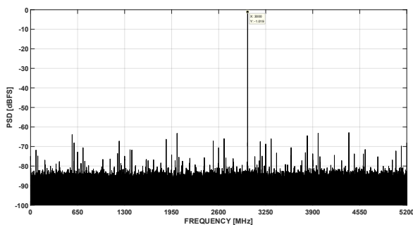
图 7-9. FFT at F_{in} = 3\text{GHz} , 10.4GSPS (0.5Vpp FS, -1 dBFS)
