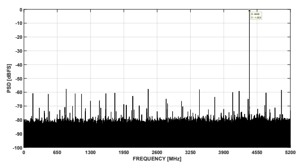
图 7-12. FFT at Fin = 6GHz, 10.4GSPS (0.5Vpp FS, -1 dBFS)
