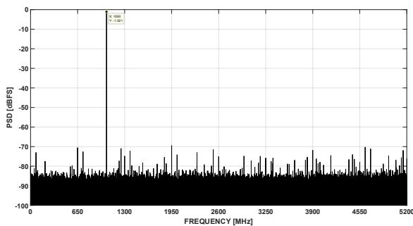
图 7-7. FFT at F_{in} = 1.05\text{GHz} , 10.4GSPS (0.5Vpp FS, -1 dBFS)
