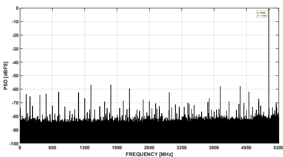
图 7-25. FFT at Fin = 5GHz, 10.4GSPS (0.8Vpp FS, -1 dBFS)
