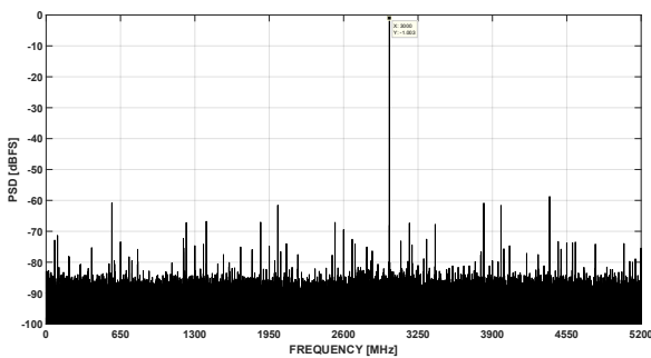
图 7-23. FFT at Fin = 3GHz, 10.4GSPS (0.8Vpp FS, -1 dBFS)
