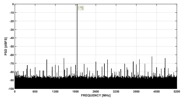
图 7-22. FFT at Fin = 2GHz, 10.4GSPS (0.8Vpp FS, -1 dBFS)
