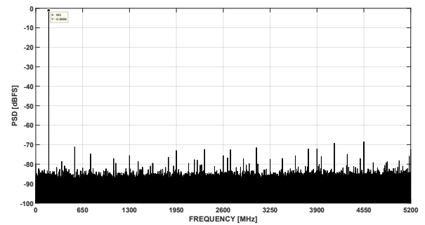
图 7-6. FFT at F_{in} = 180\text{MHz} , 10.4GSPS (0.5Vpp FS, -1 dBFS)
