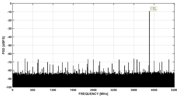
图 7-19. FFT at Fin = 6GHz, 10.4GSPS (0.5Vpp FS, -10 dBFS)
