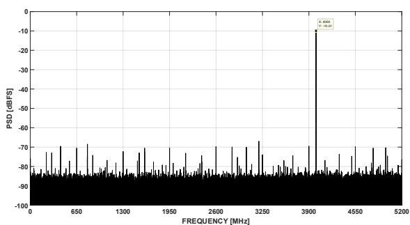
图 7-17. FFT at Fin = 4GHz, 10.4GSPS (0.5Vpp FS, -10 dBFS)
