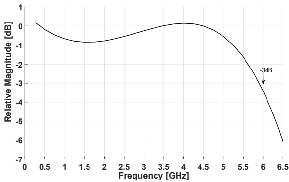
图 7-5. Relative Magnitude vs Input Frequency
