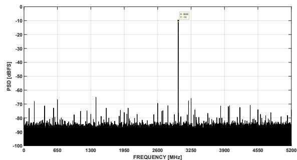
图 7-16. FFT at Fin = 3GHz, 10.4GSPS (0.5Vpp FS, -10 dBFS)
