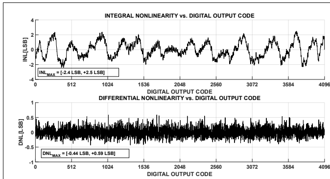
图 7-3. INL/DNL at F_{in} = 180\text{MHz} , 10.4GSPS (0.5Vpp FS)
