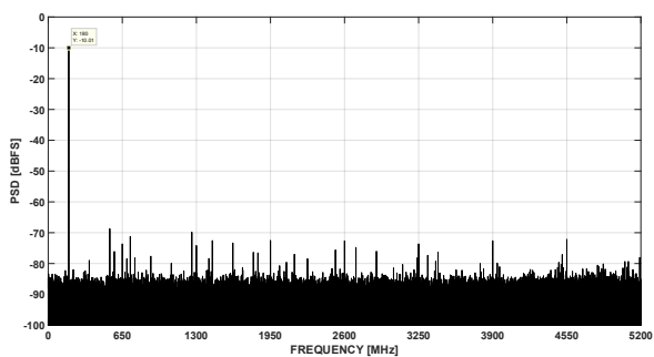
图 7-13. FFT at Fin = 180MHz, 10.4GSPS (0.5Vpp FS, -10 dBFS)
