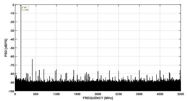
图 7-20. FFT at Fin = 180MHz, 10.4GSPS (0.8Vpp FS, -1 dBFS)
